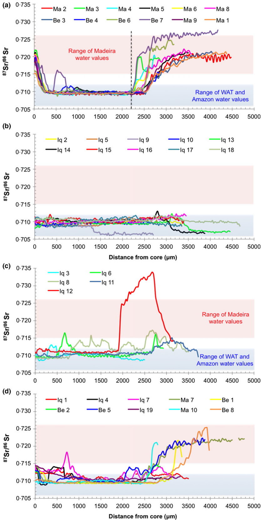
Fig. 3. Laser ablation-MC-ICPMS transects of ^{87}\text{Sr}/^{86}\text{Sr} along otolith transverse sections (from the core to the edge) of Brachyplatystoma rousseauxii . Each curve corresponds to one individual caught either in the upper Madeira (Mamoré, Ma and Beni, Be rivers) or in the upper Amazon (fish landed in Iquitos, Iq; see Fig. 1). Four migratory patterns were identified among transects (a, b, c, d, see text). The dashed line (a) represents the size at first sexual maturity of B. rousseauxii in the Madeira basin (Fig. S2).
